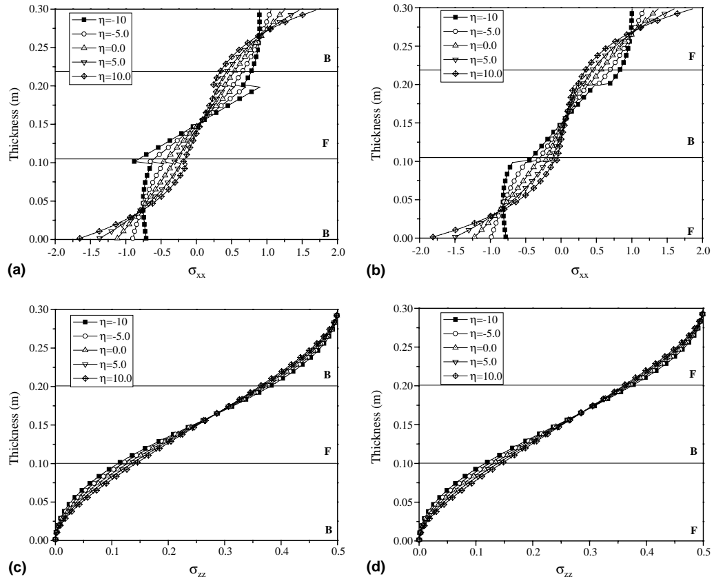
Fig. 5. Stress component distribution \sigma_{xx} and \sigma_{zz} (N/m 2 ) across the thickness direction: \sigma_{xx} in (a) and \sigma_{zz} in (c) for the B/F/B, and \sigma_{xx} in (b) and \sigma_{zz} in (d) for F/B/F case.
